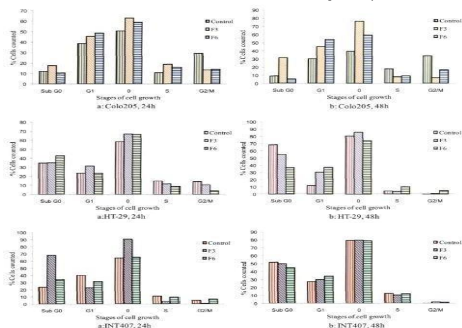
Figure 2. (a-f) Depict the effect of exposure to IC 50 concentrations of fractions 3 and 6 on the three cell lines.
