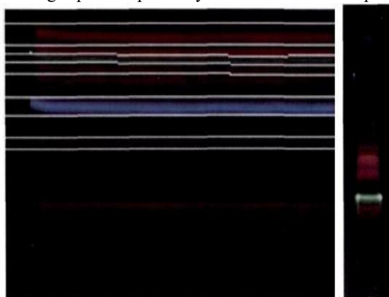
Figure 1. (a) Photo documentation of DCM extract (b) Photo image of LB test for steroidal nucleus
