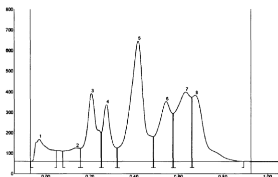
Figure 1. (c) HPTLC finger-print of DCM extract.
