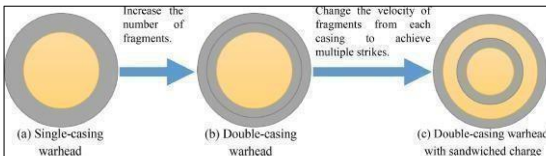
Figure 1. Warhead employment in bomblet [15].
