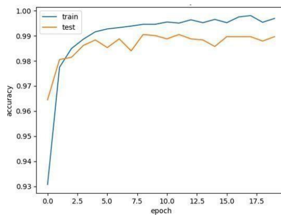
Figure 11. Model Accuracy (outcome of this study).
