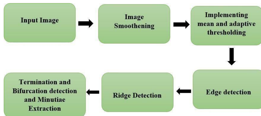
Figure 2. Overall research design used in this study (Based on the implementation of this study).
