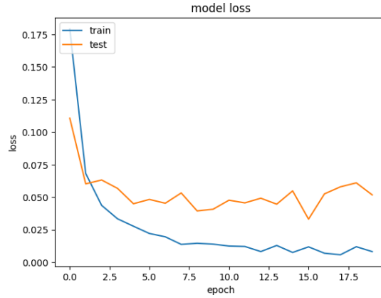
Figure 12. Model Loss (outcome of this study).
