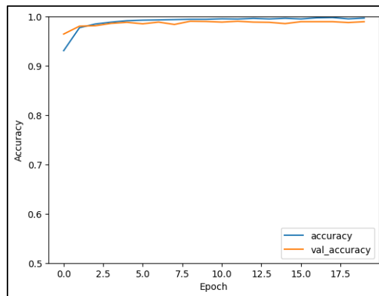
Figure 10. Accuracy and validation accuracy of the proposed model (outcome of this study).
