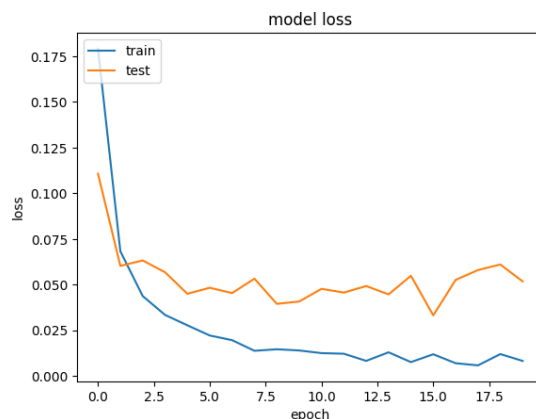
Fig. 12. Model Loss (outcome of this study)
