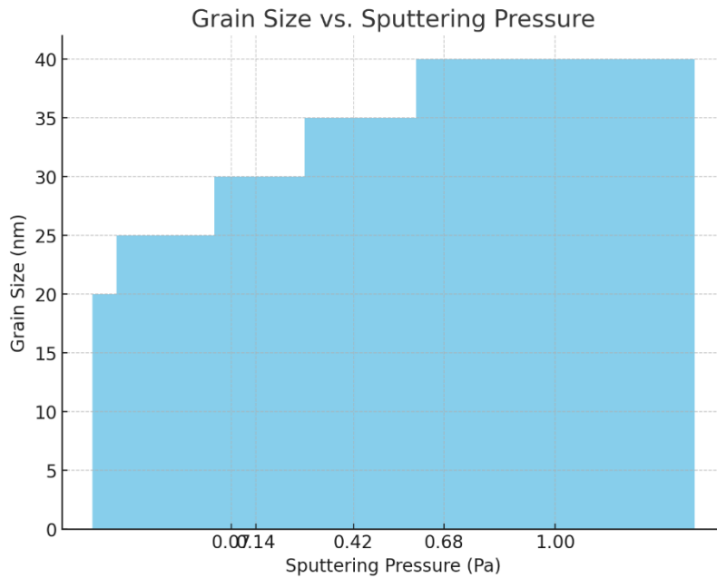
Fig. 1. Grain Size vs. Sputtering Pressure
